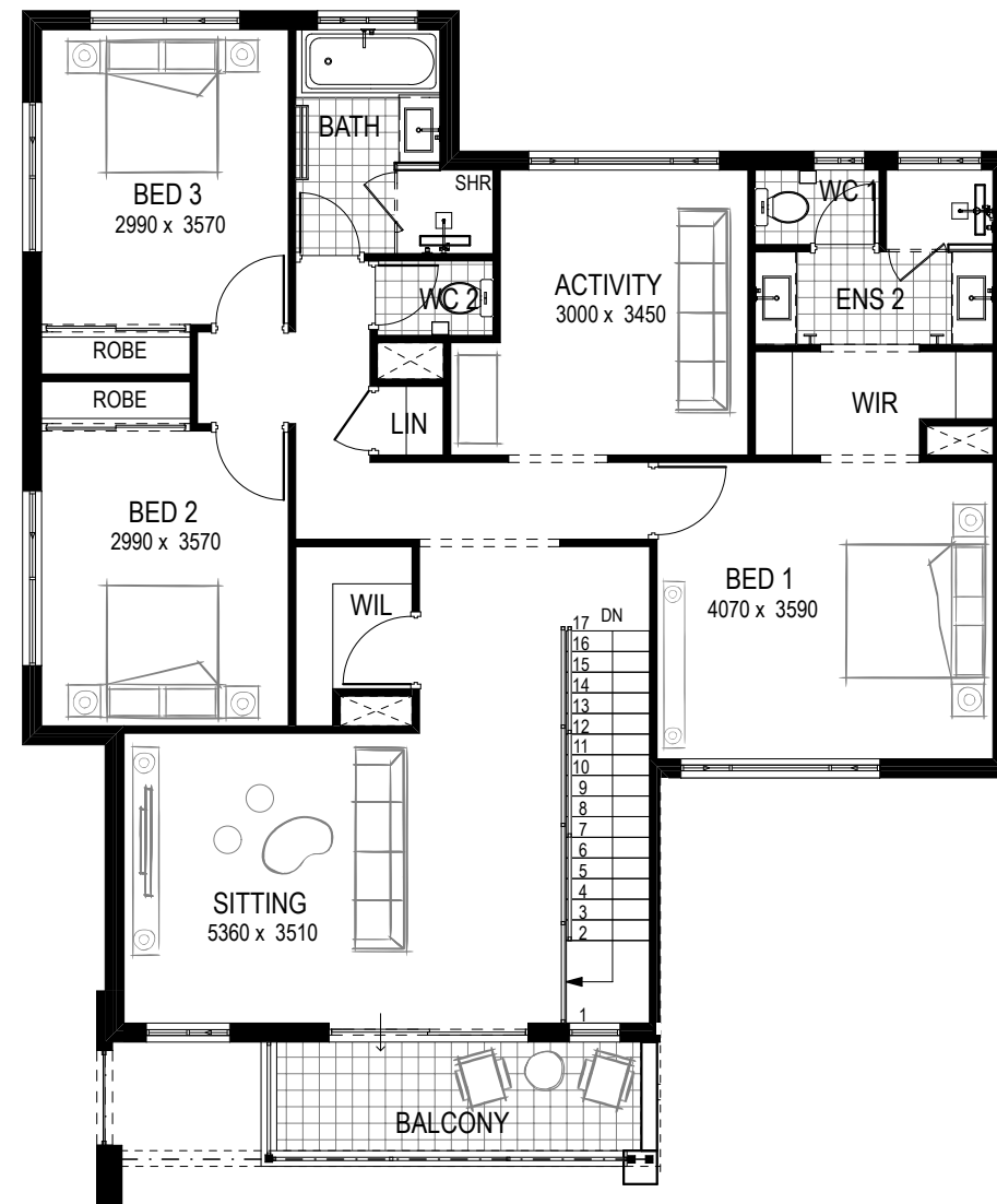
UPPER FLOOR PLAN SCALE 1:100
